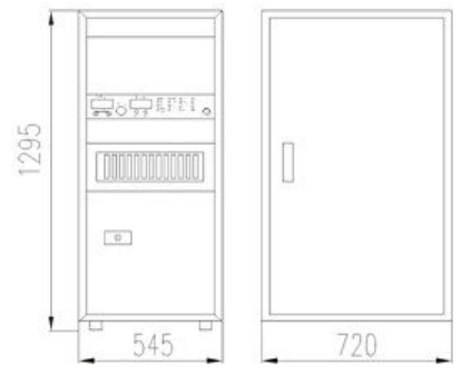
Power Amplifier DA-2
