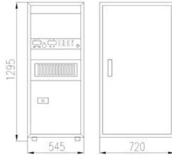
Power Amplifier DA-2/3
