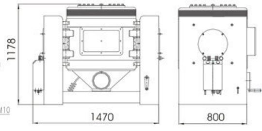
Shaker ET-30-550
