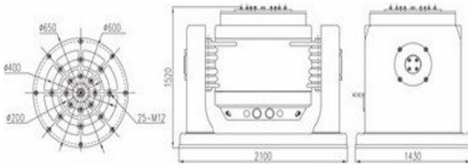
Shaker ET-200-650
