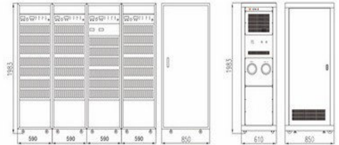
Power Amplifier DA-200
